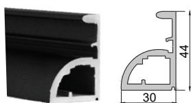
Handle Profile
