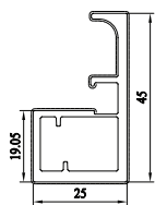
Handle Profile Profile Length: 3000mm
