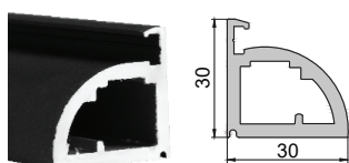
Frame Profile
